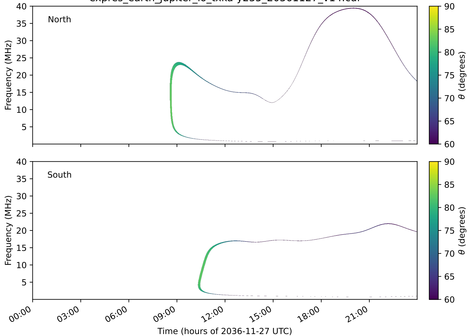
expres_earth_jupiter_io_txka-y235_20361127_v14.cdf
