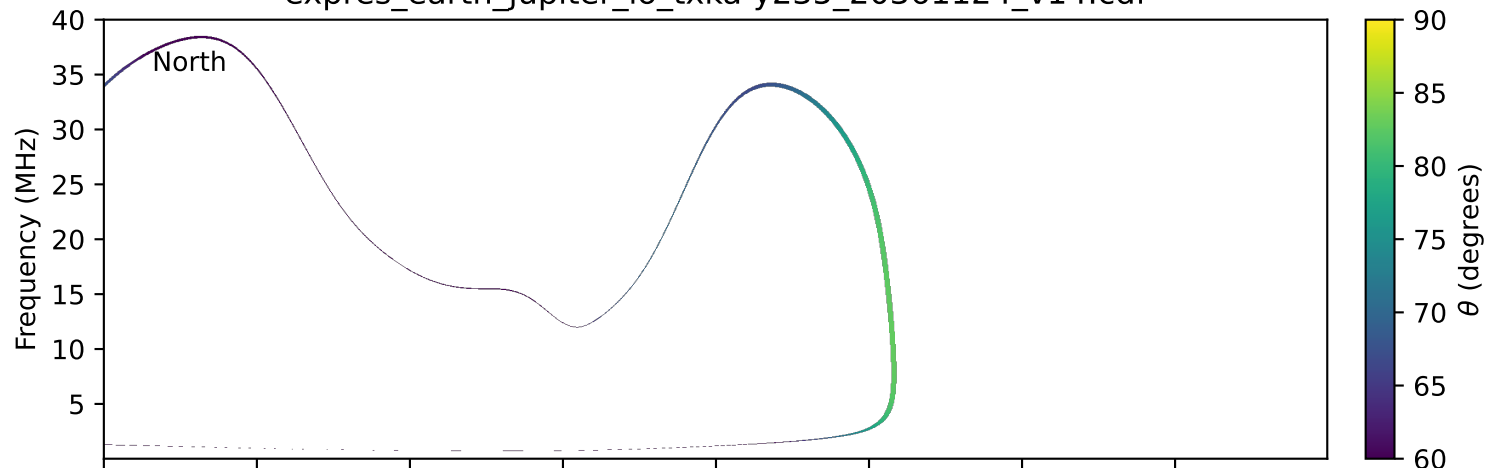
expres_earth_jupiter_io_txka-y235_20361124_v14.cdf
