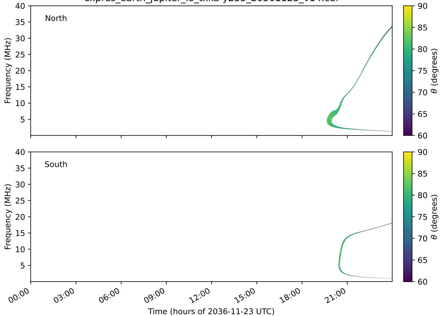
expres_earth_jupiter_io_txka-y235_20361123_v14.cdf
