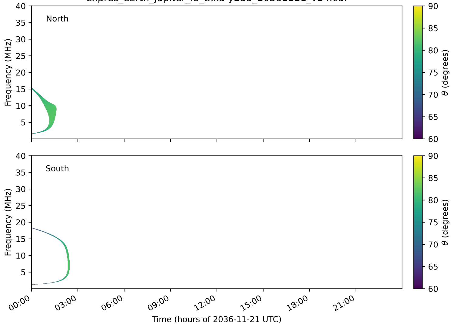
expres_earth_jupiter_io_txka-y235_20361121_v14.cdf
