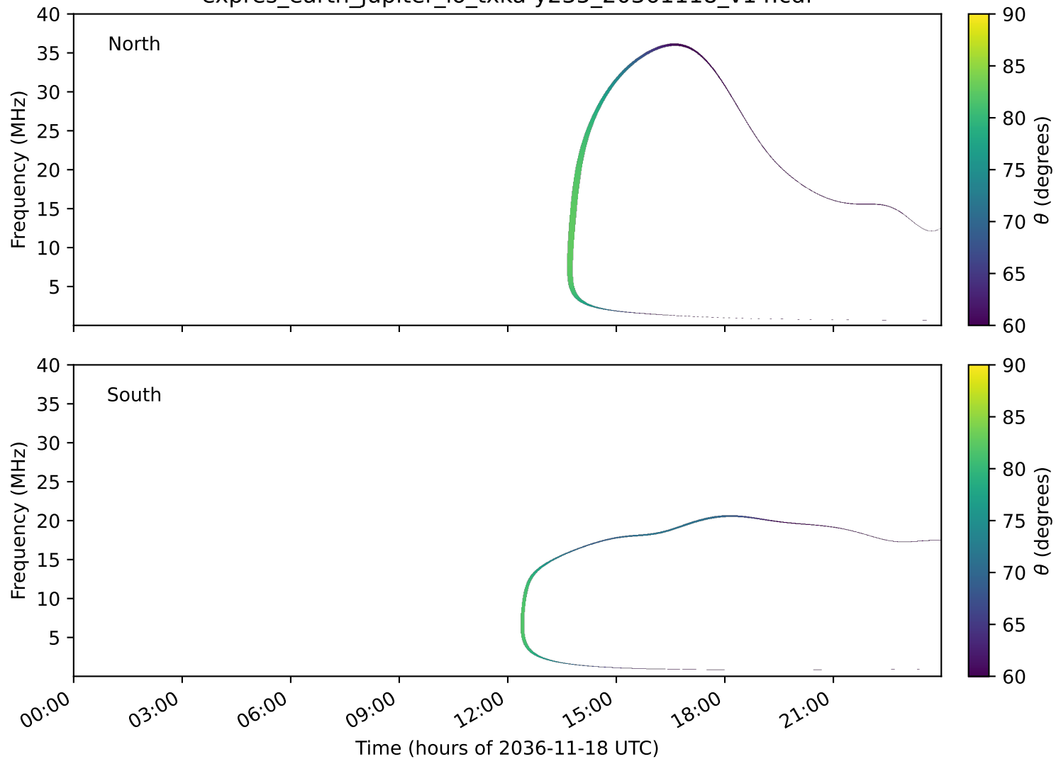
expres_earth_jupiter_io_txka-y235_20361118_v14.cdf
