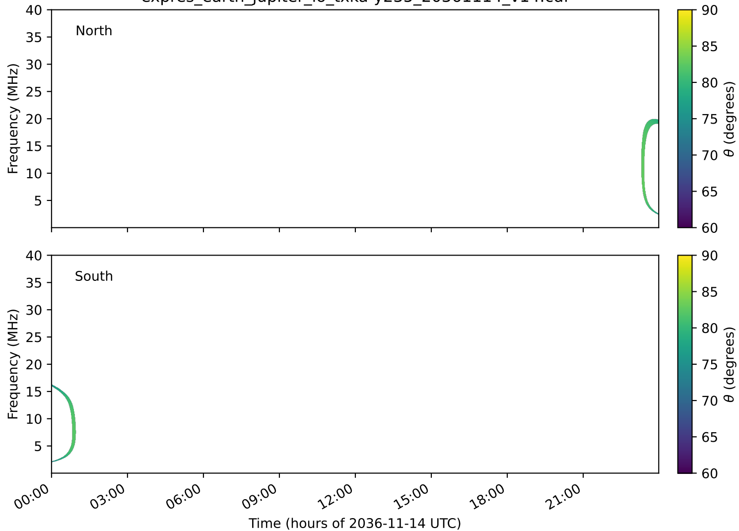
expres_earth_jupiter_io_txka-y235_20361114_v14.cdf
