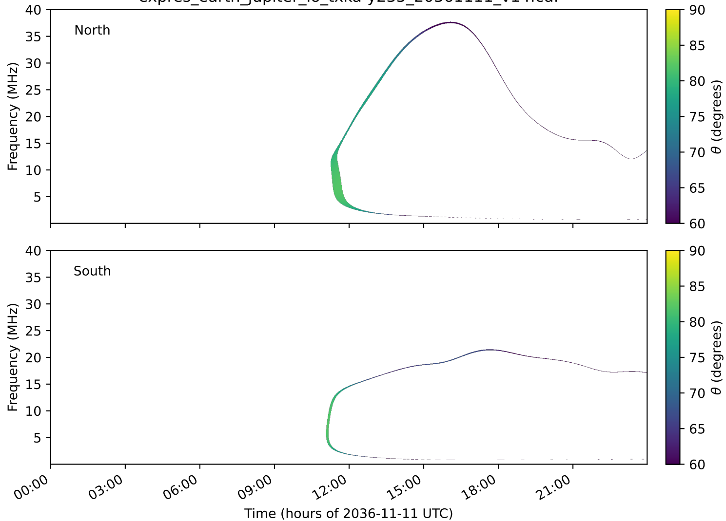
expres_earth_jupiter_io_txka-y235_20361111_v14.cdf
