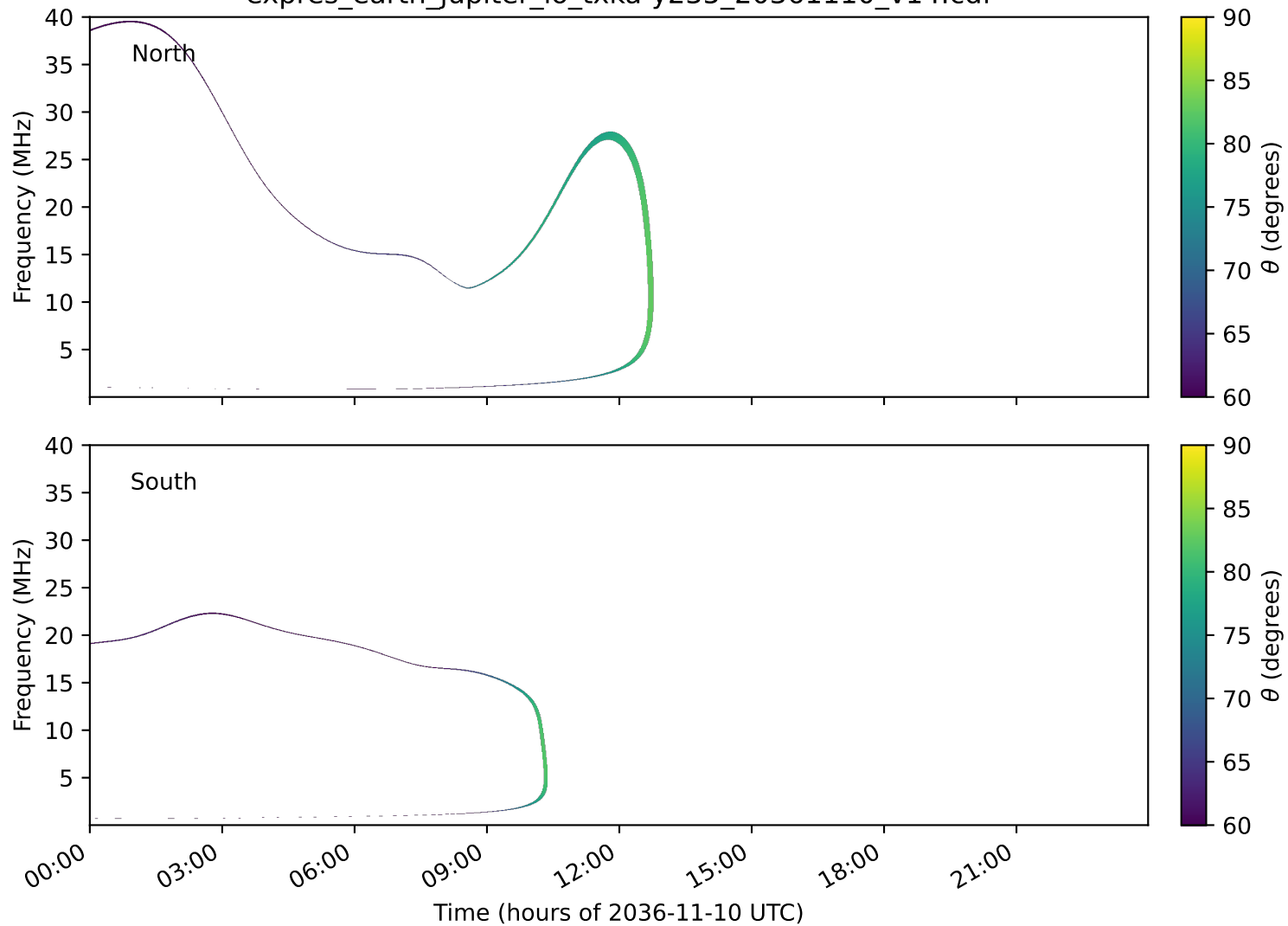
expres_earth_jupiter_io_txka-y235_20361110_v14.cdf
