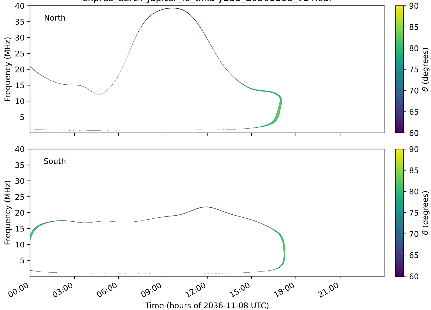
expres_earth_jupiter_io_txka-y235_20361108_v14.cdf
