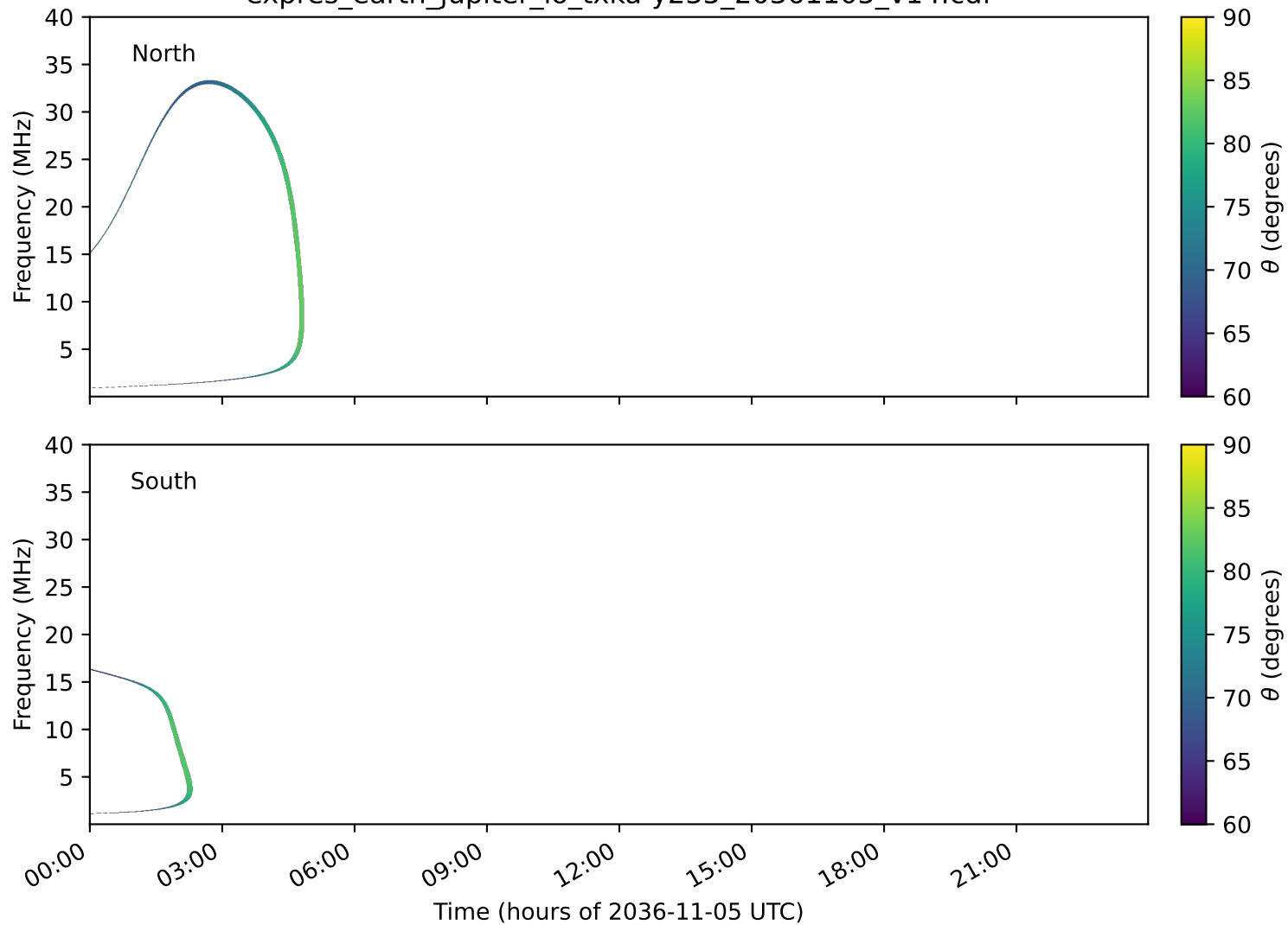
expres_earth_jupiter_io_txka-y235_20361105_v14.cdf
