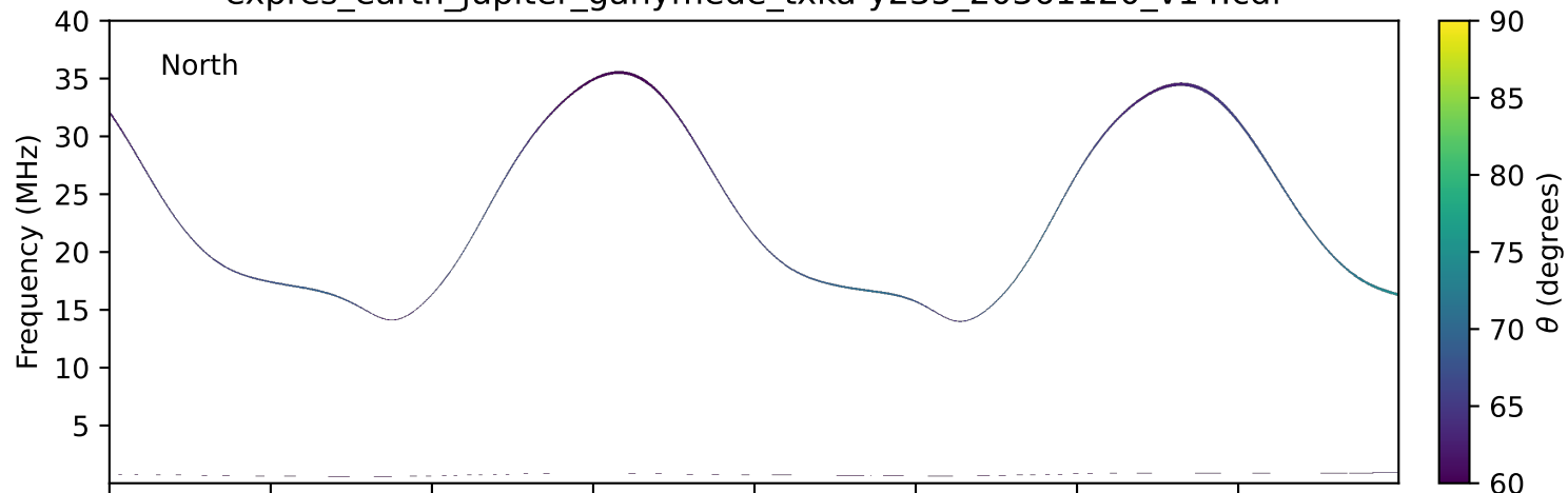
expres_earth_jupiter_ganymede_txka-y235_20361120_v14.cdf
