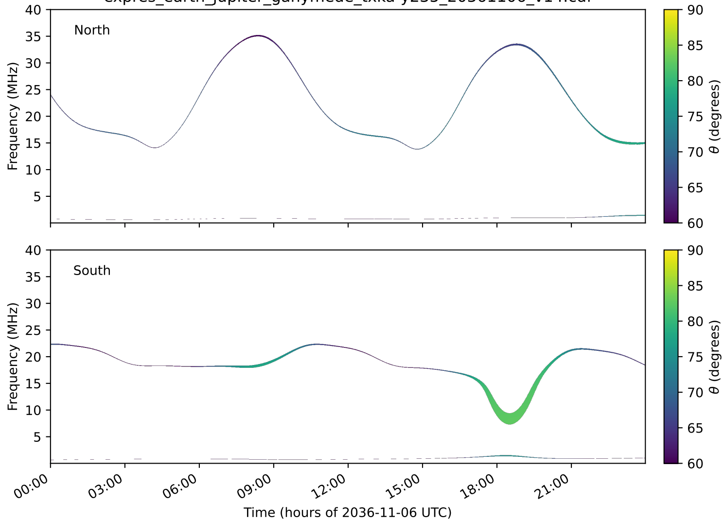
expres_earth_jupiter_ganymede_txka-y235_20361106_v14.cdf
