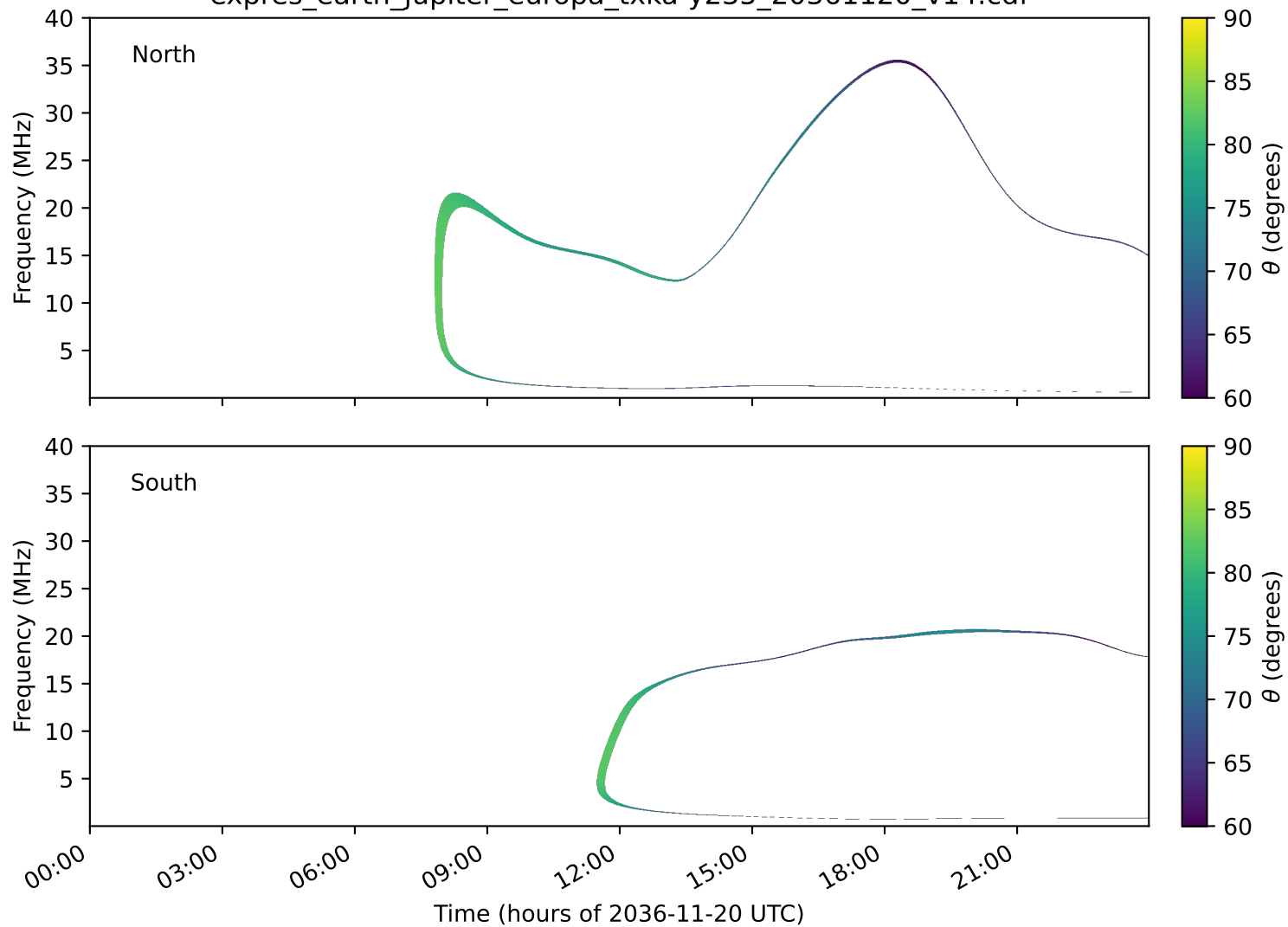
expres_earth_jupiter_europa_txka-y235_20361120_v14.cdf
