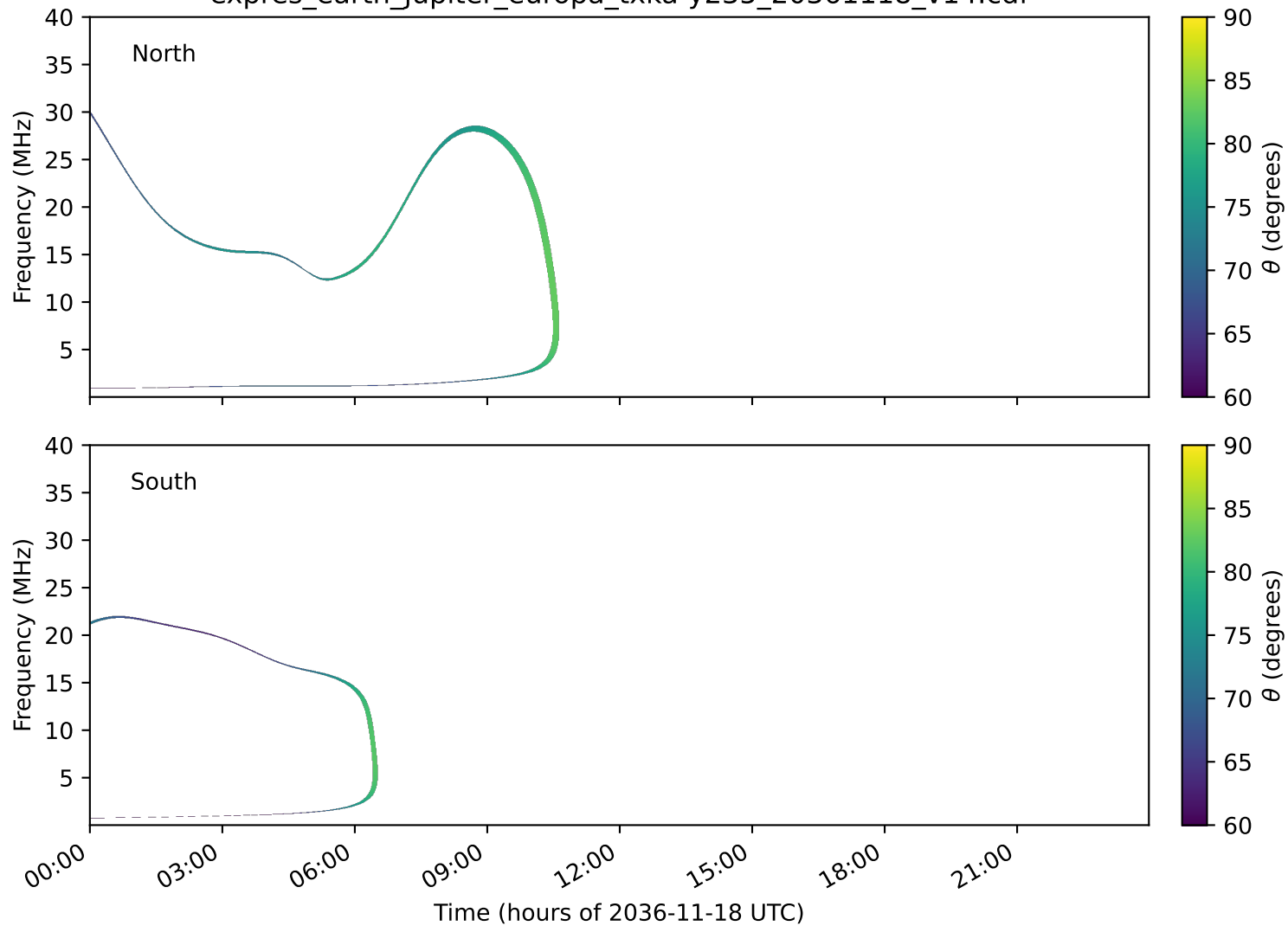
expres_earth_jupiter_europa_txka-y235_20361118_v14.cdf
