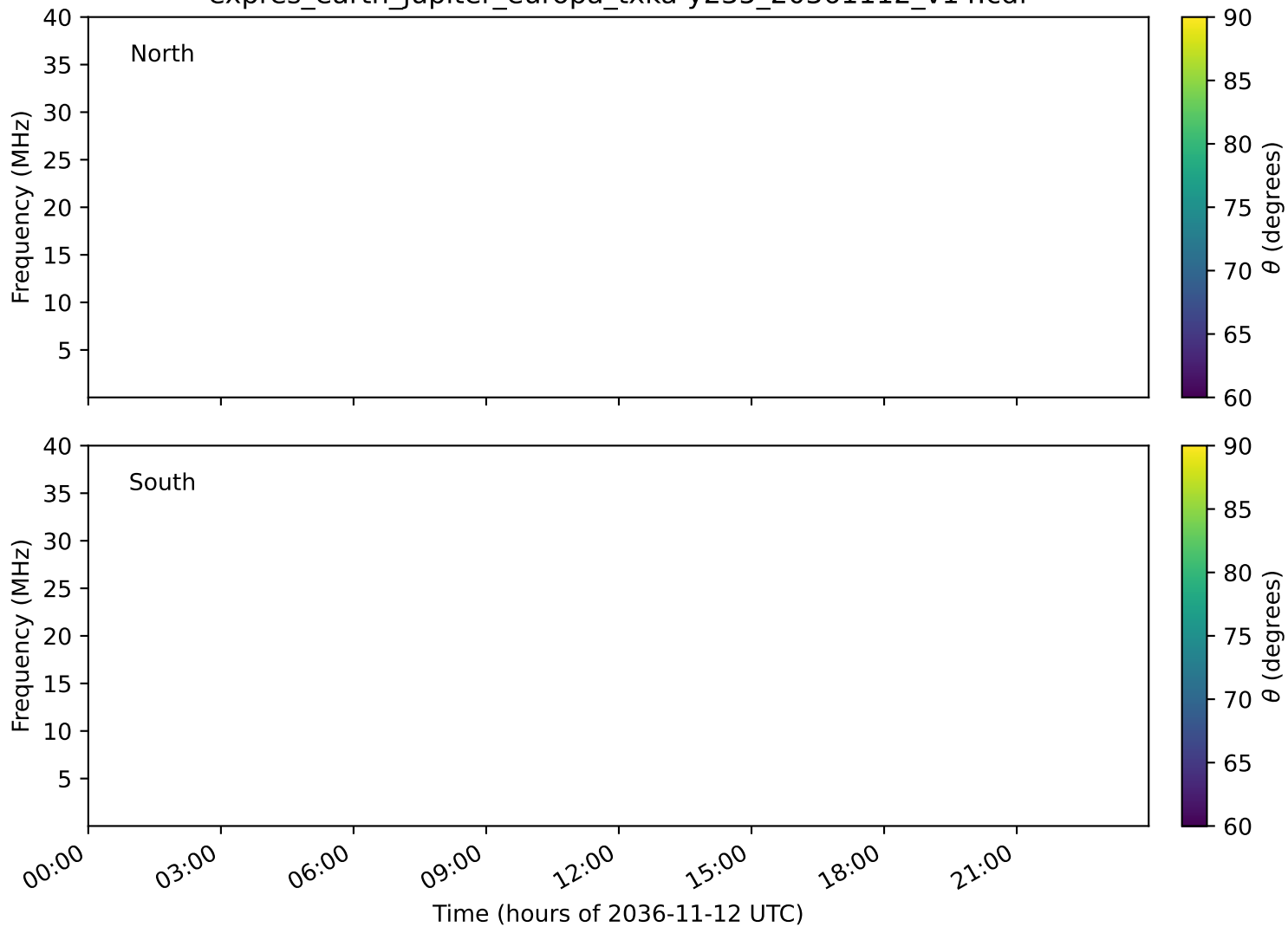
expres_earth_jupiter_europa_txka-y235_20361112_v14.cdf
