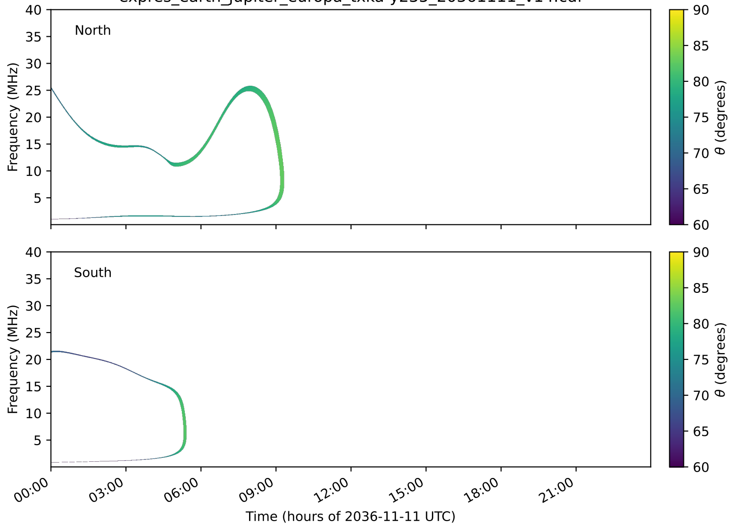
expres_earth_jupiter_europa_txka-y235_20361111_v14.cdf
