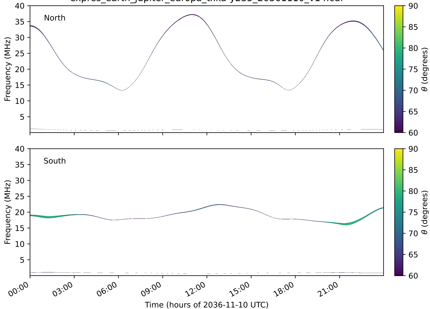
expres_earth_jupiter_europa_txka-y235_20361110_v14.cdf
