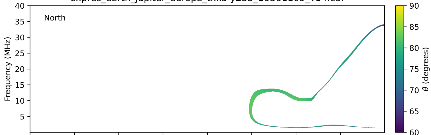
expres_earth_jupiter_europa_txka-y235_20361109_v14.cdf
