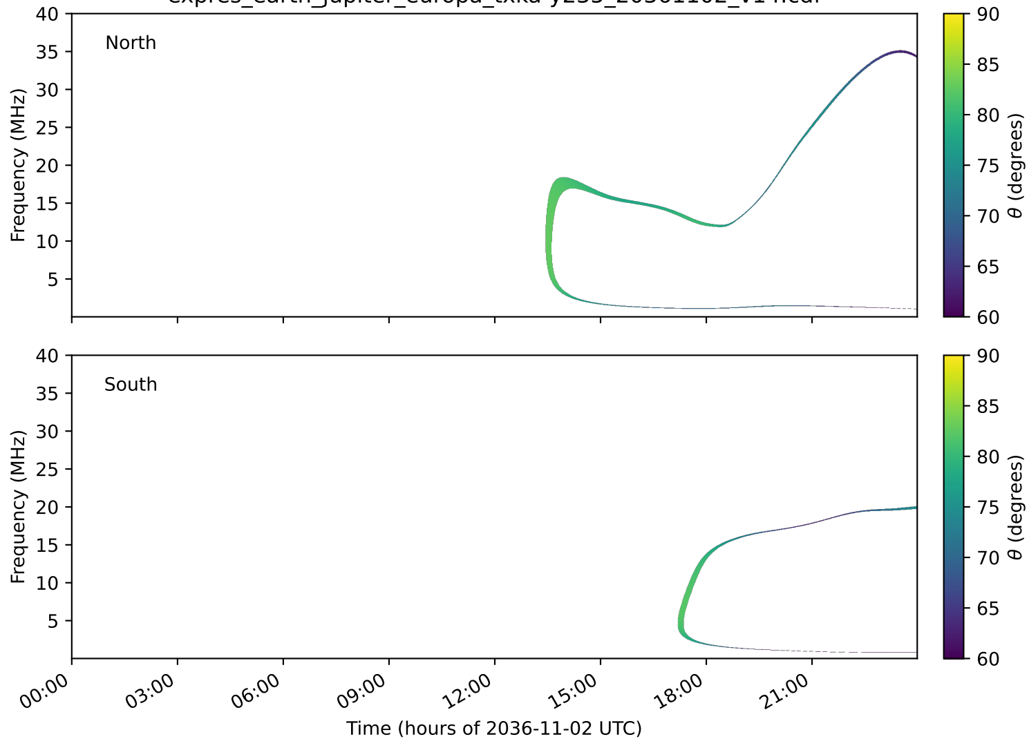
expres_earth_jupiter_europa_txka-y235_20361102_v14.cdf
