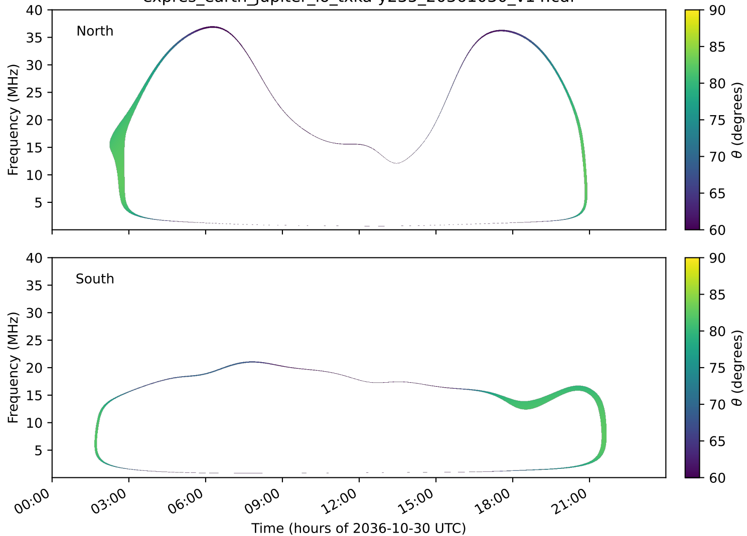
expres_earth_jupiter_io_txka-y235_20361030_v14.cdf
