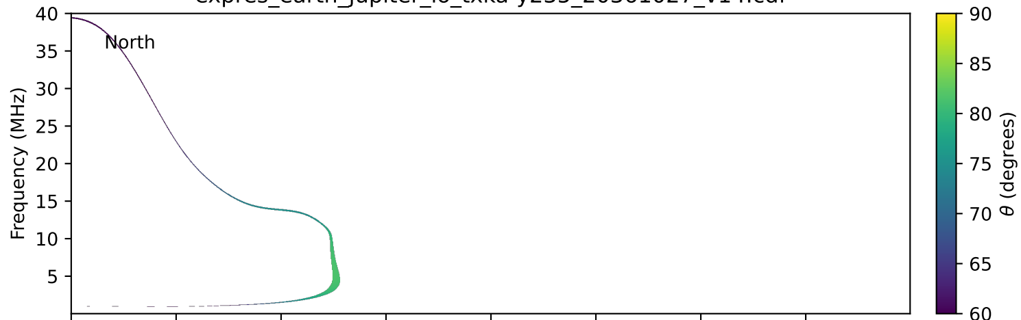
expres_earth_jupiter_io_txka-y235_20361027_v14.cdf
