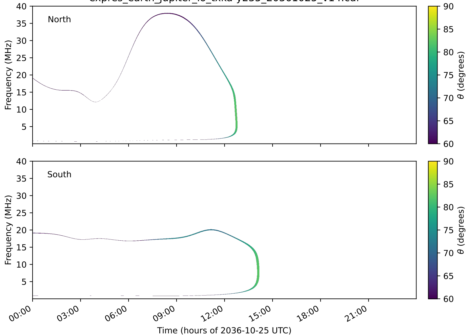
expres_earth_jupiter_io_txka-y235_20361025_v14.cdf
