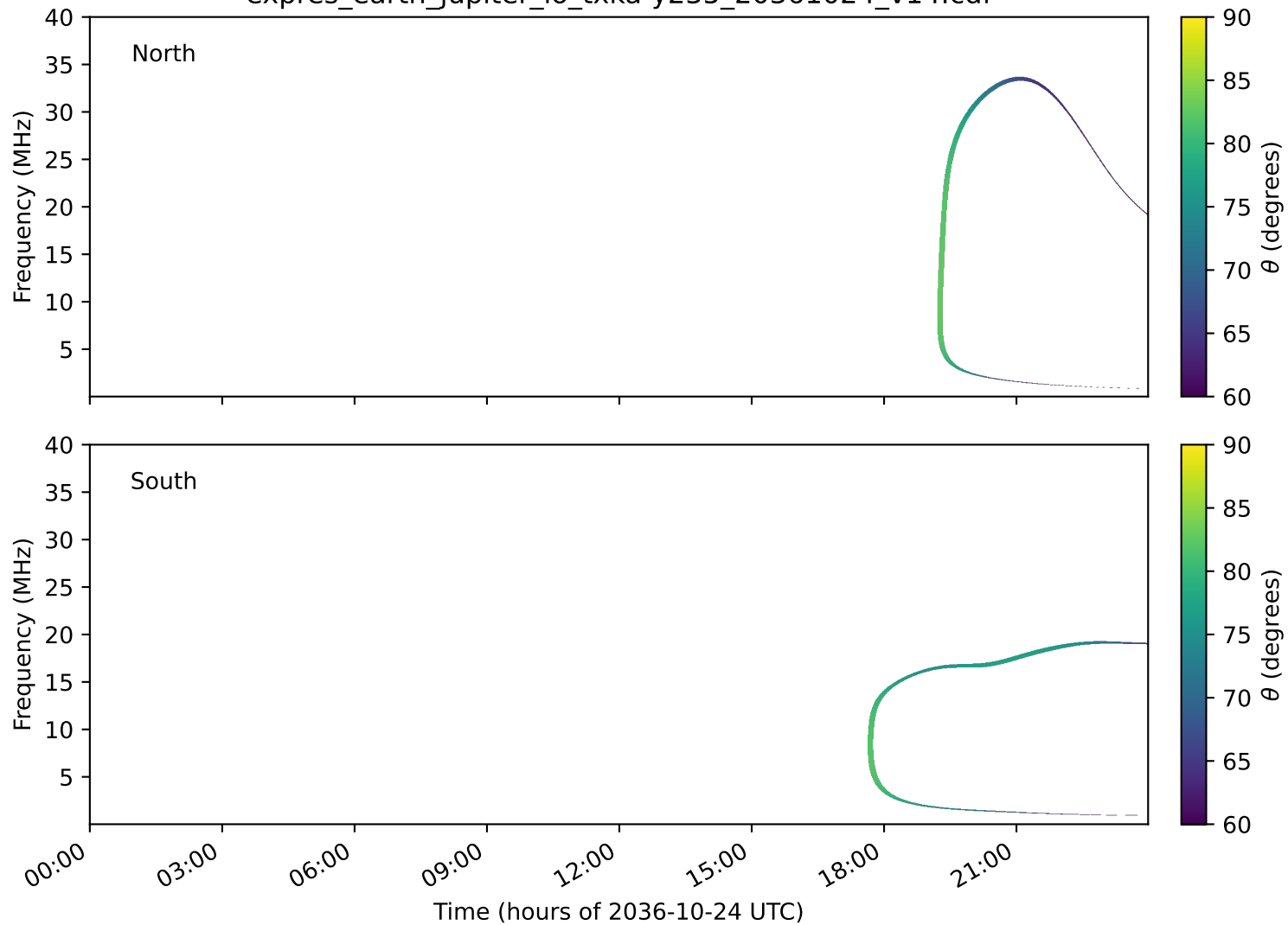
expres_earth_jupiter_io_txka-y235_20361024_v14.cdf
