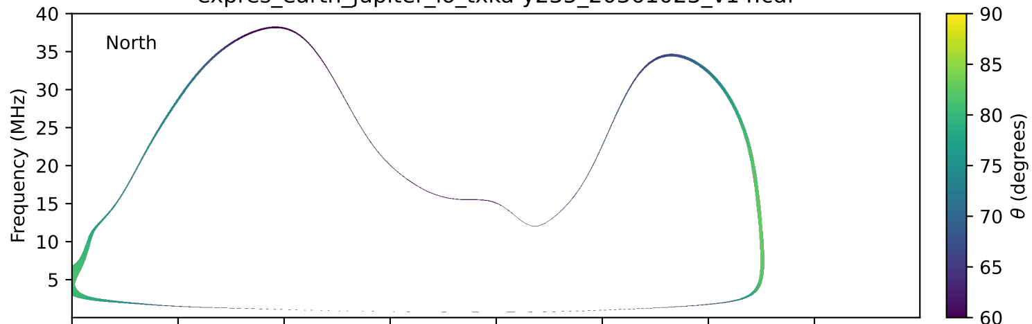
expres_earth_jupiter_io_txka-y235_20361023_v14.cdf
