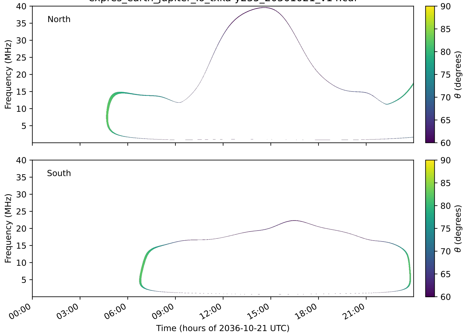
expres_earth_jupiter_io_txka-y235_20361021_v14.cdf
