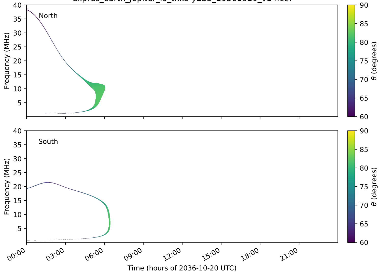
expres_earth_jupiter_io_txka-y235_20361020_v14.cdf
