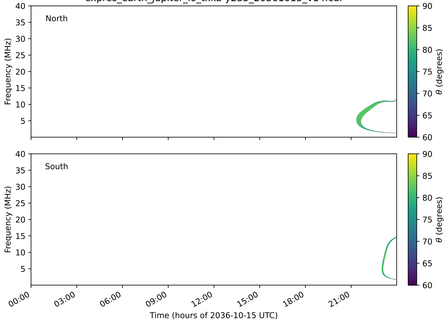
expres_earth_jupiter_io_txka-y235_20361015_v14.cdf
