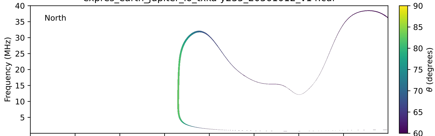
expres_earth_jupiter_io_txka-y235_20361012_v14.cdf
