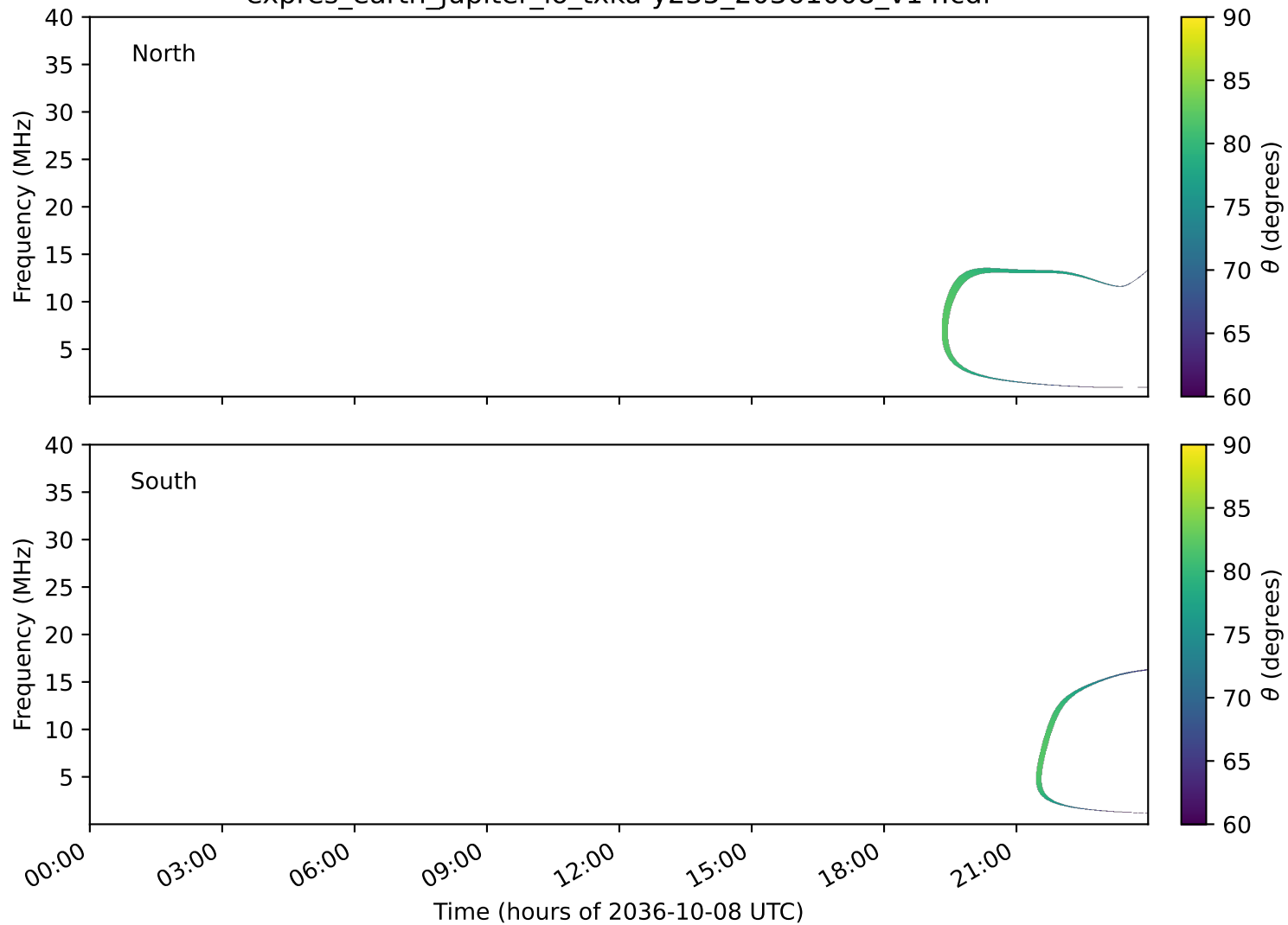
expres_earth_jupiter_io_txka-y235_20361008_v14.cdf
