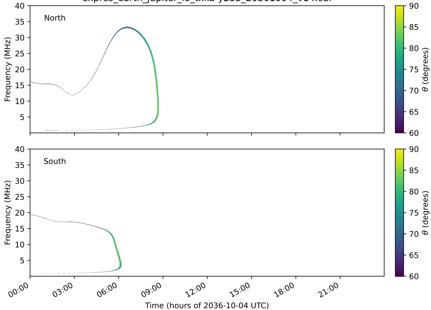
expres_earth_jupiter_io_txka-y235_20361004_v14.cdf
