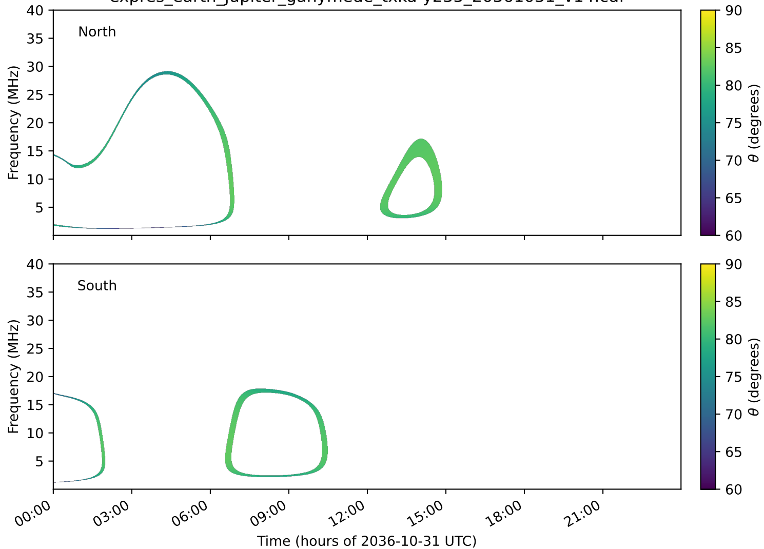
expres_earth_jupiter_ganymede_txka-y235_20361031_v14.cdf
