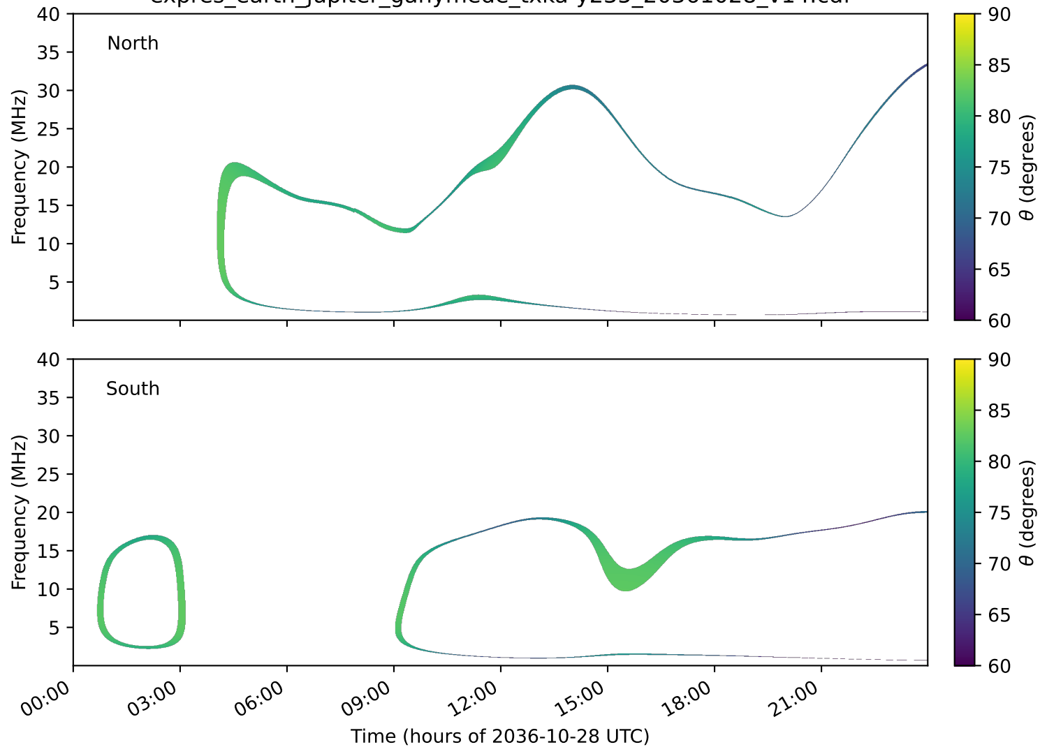
expres_earth_jupiter_ganymede_txka-y235_20361028_v14.cdf
