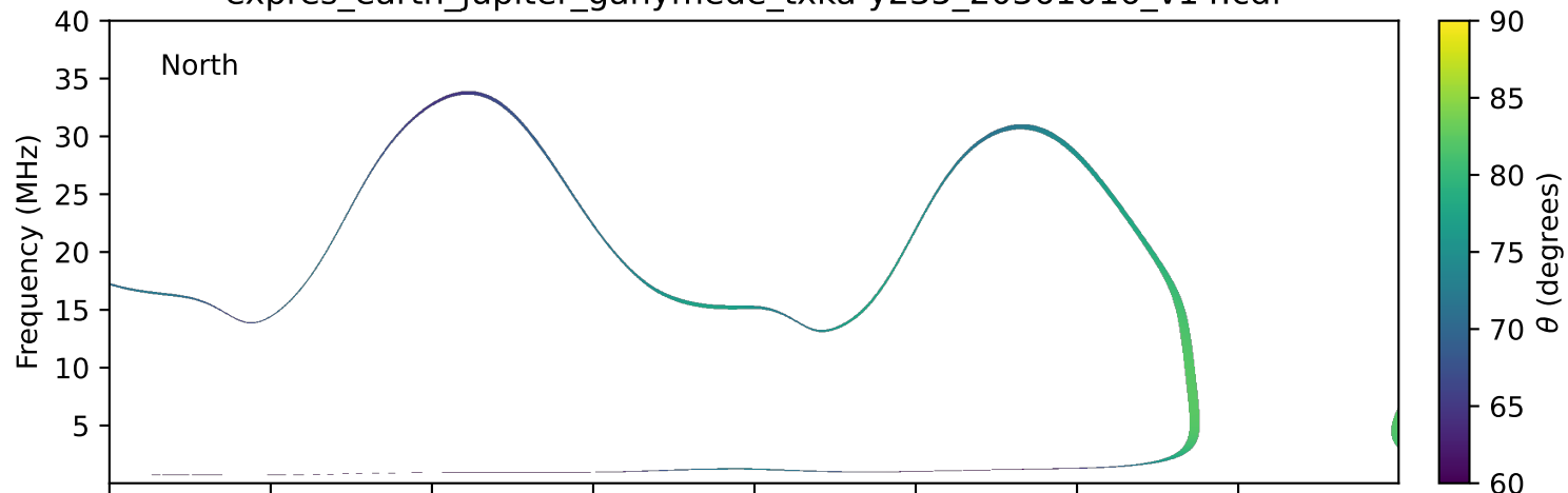
expres_earth_jupiter_ganymede_txka-y235_20361016_v14.cdf
