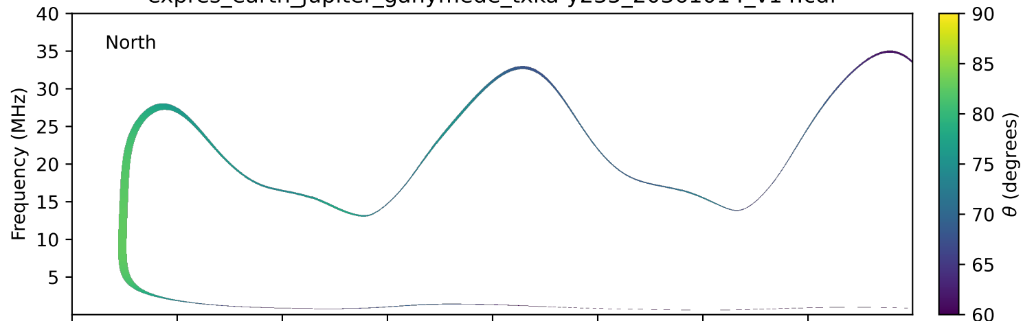
expres_earth_jupiter_ganymede_txka-y235_20361014_v14.cdf
