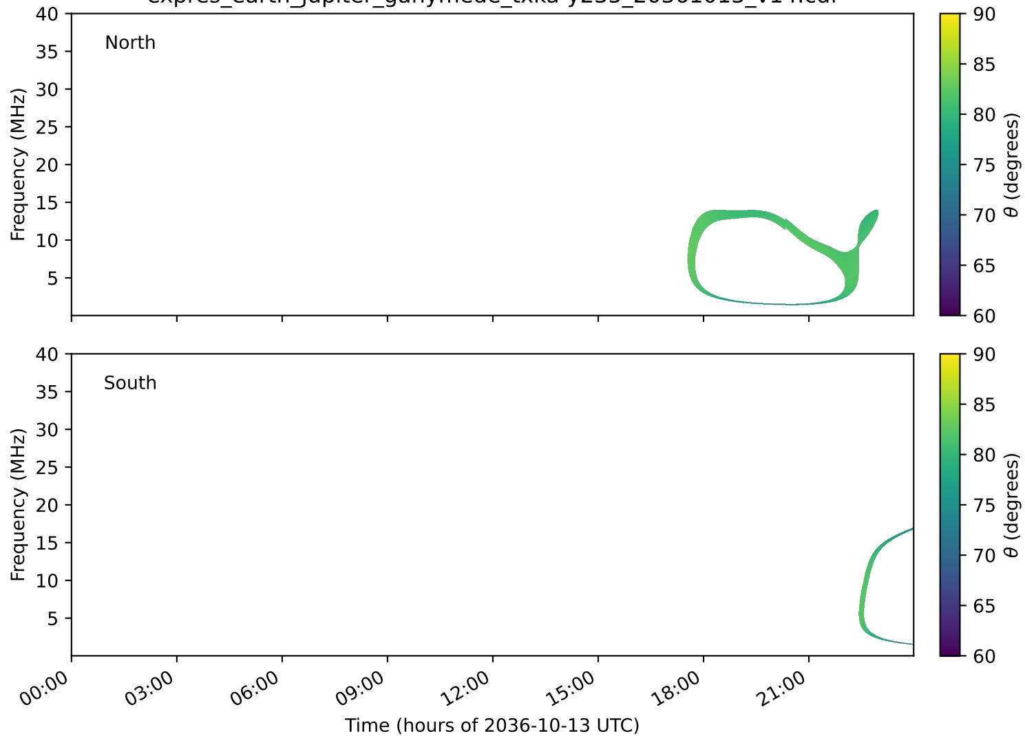
expres_earth_jupiter_ganymede_txka-y235_20361013_v14.cdf
