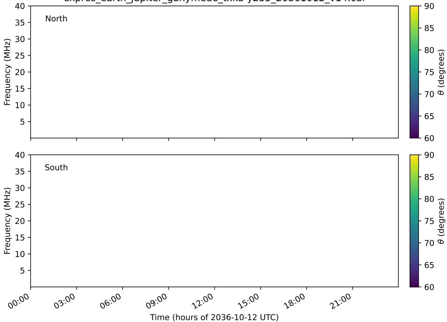
expres_earth_jupiter_ganymede_txka-y235_20361012_v14.cdf
