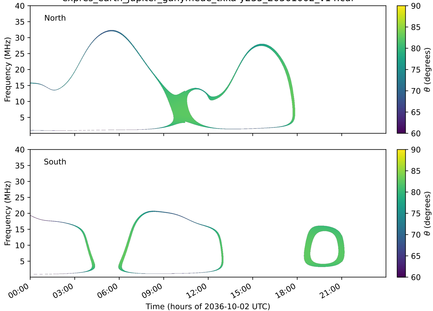
expres_earth_jupiter_ganymede_txka-y235_20361002_v14.cdf
