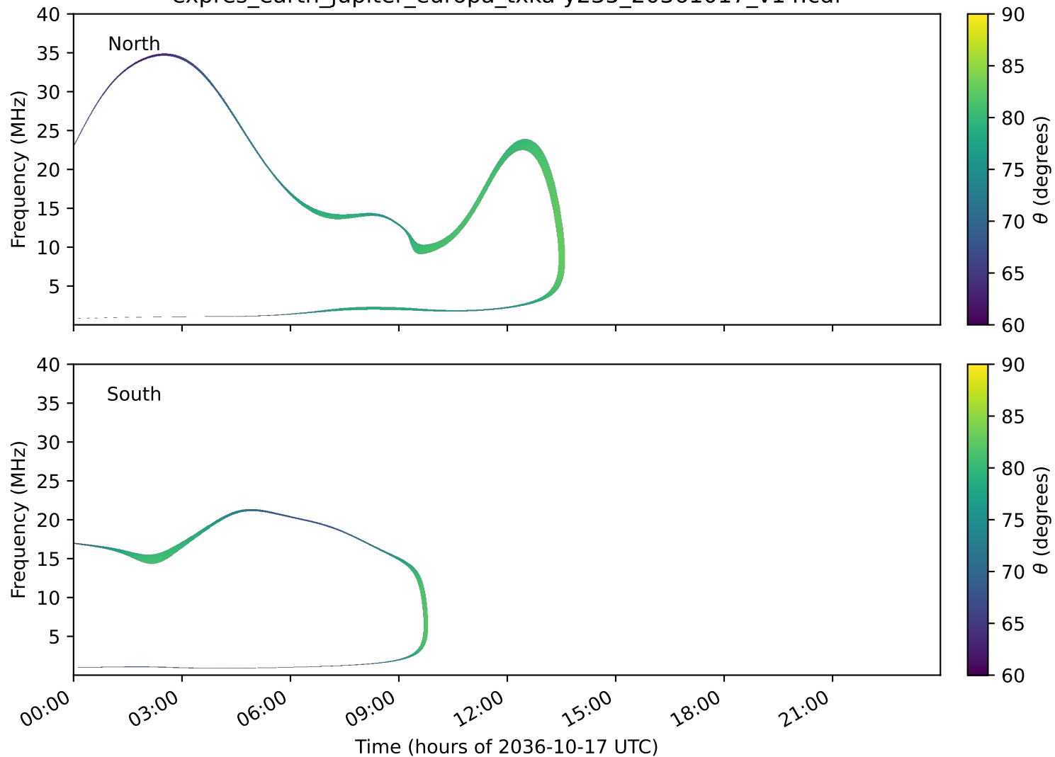
expres_earth_jupiter_europa_txka-y235_20361017_v14.cdf
