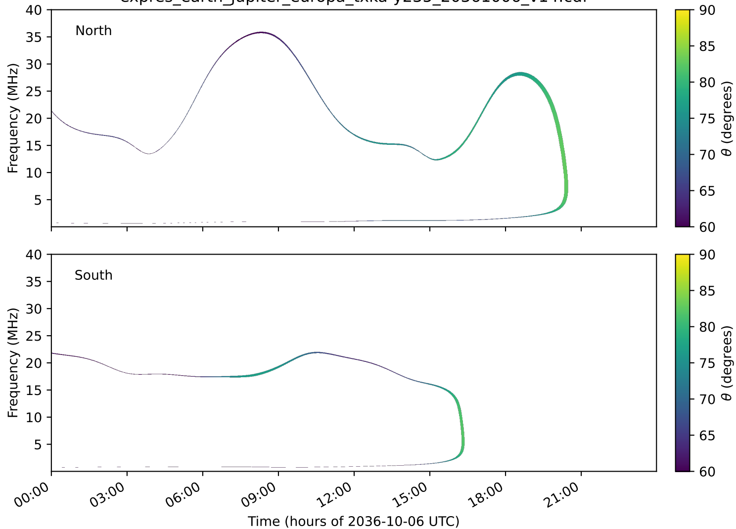
expres_earth_jupiter_europa_txka-y235_20361006_v14.cdf
