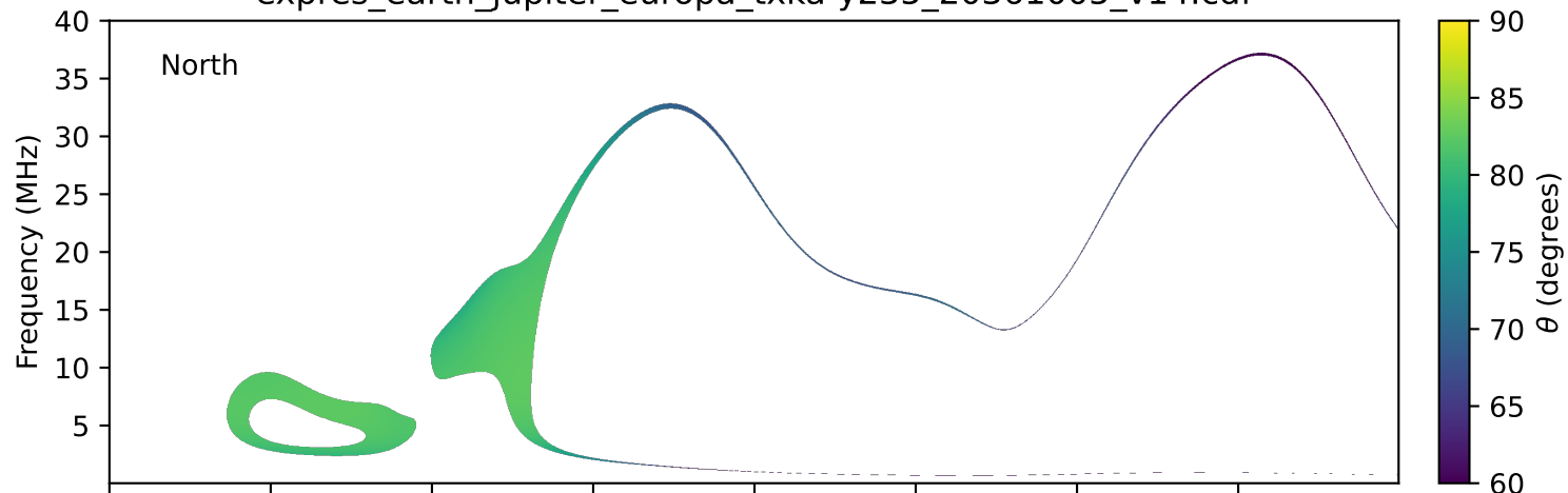
expres_earth_jupiter_europa_txka-y235_20361005_v14.cdf
