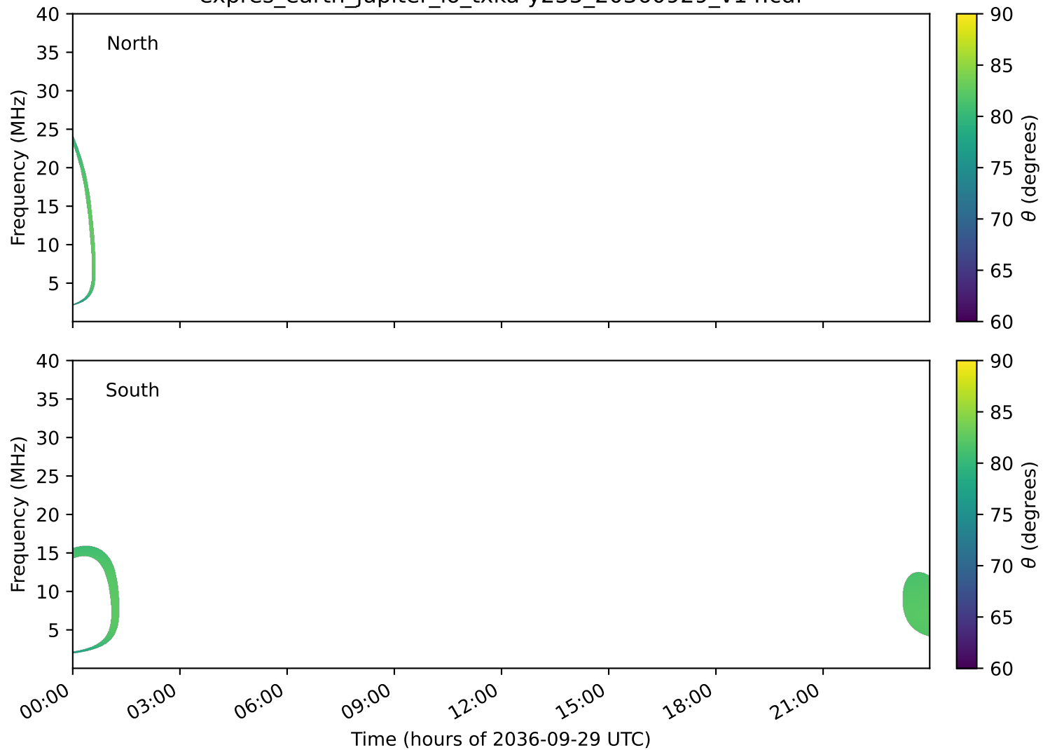
expres_earth_jupiter_io_txka-y235_20360929_v14.cdf
