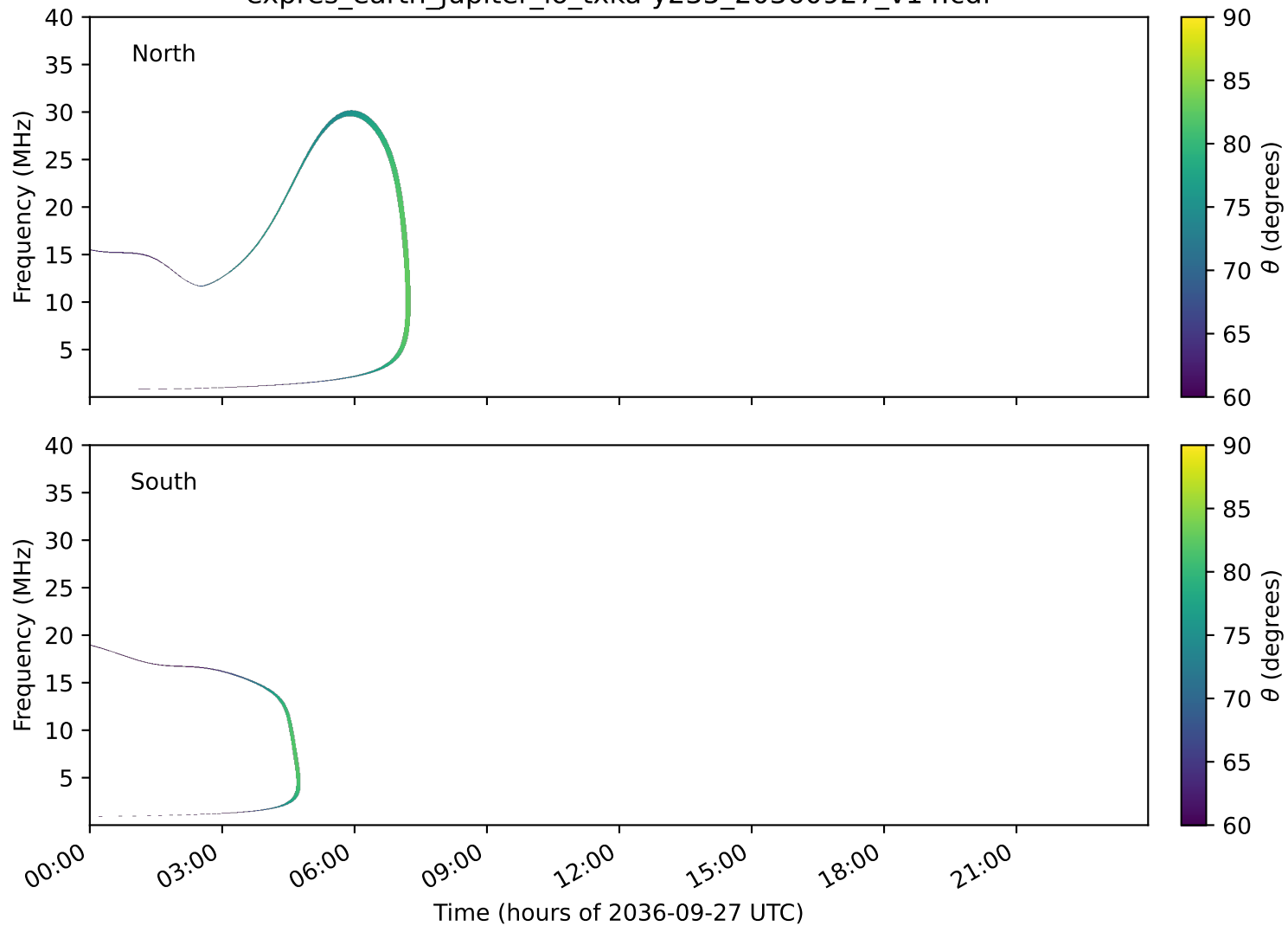
expres_earth_jupiter_io_txka-y235_20360927_v14.cdf
