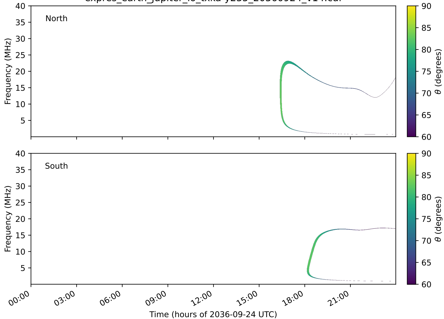
expres_earth_jupiter_io_txka-y235_20360924_v14.cdf
