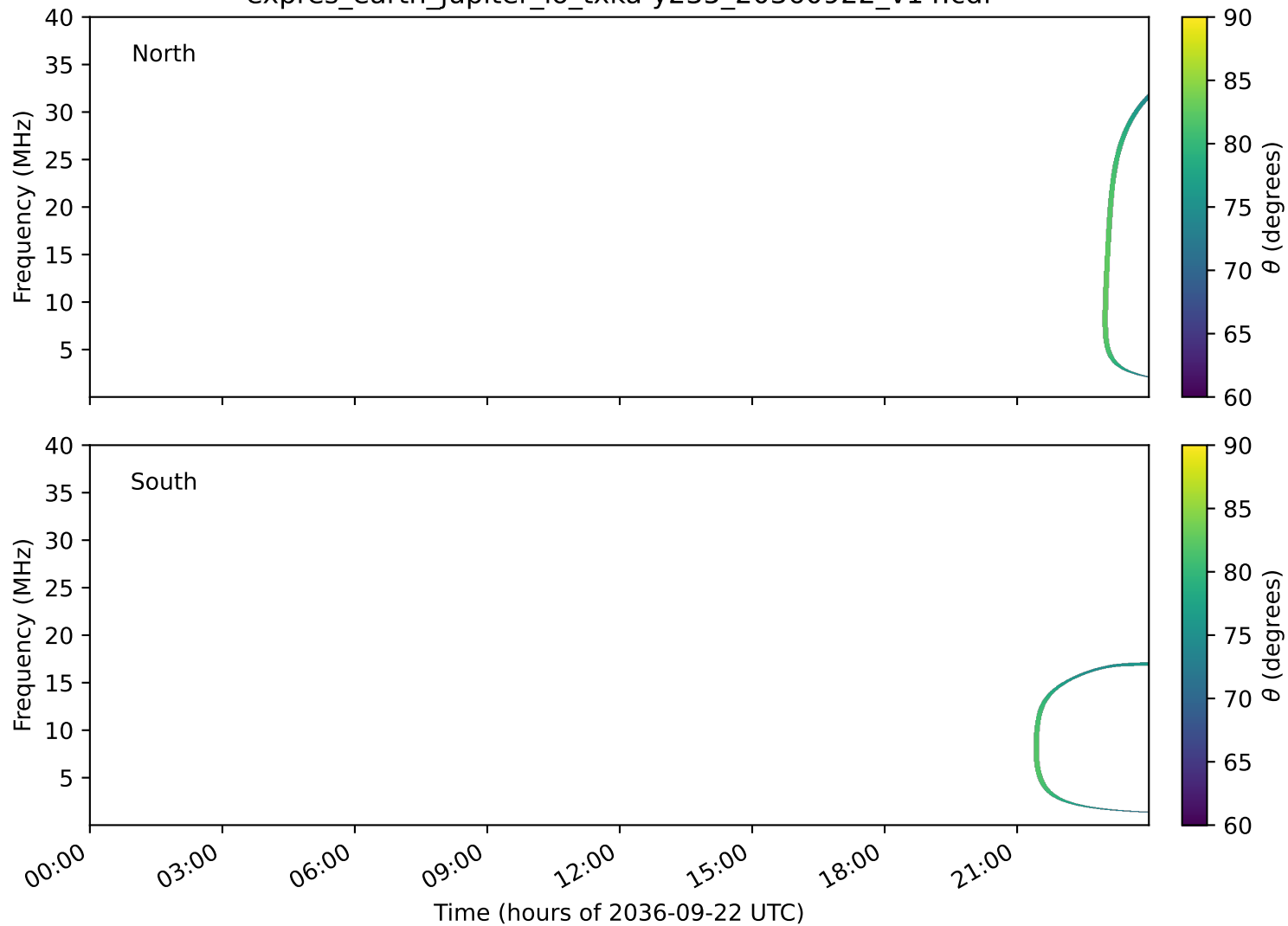
expres_earth_jupiter_io_txka-y235_20360922_v14.cdf
