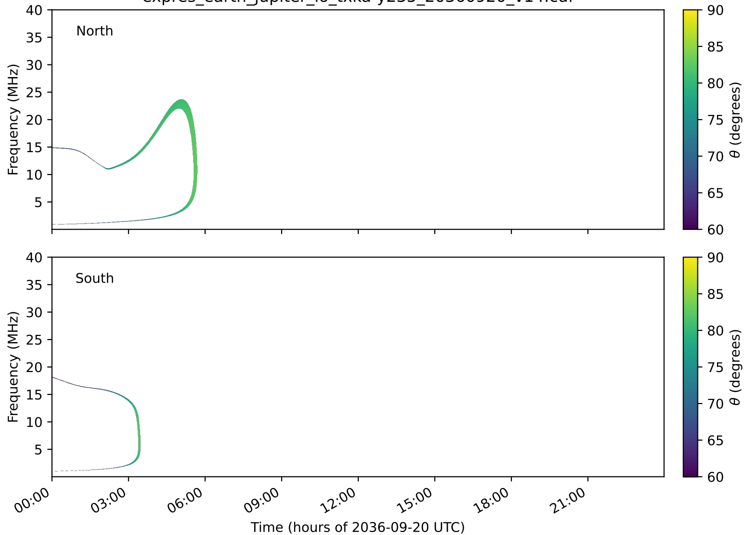
expres_earth_jupiter_io_txka-y235_20360920_v14.cdf
