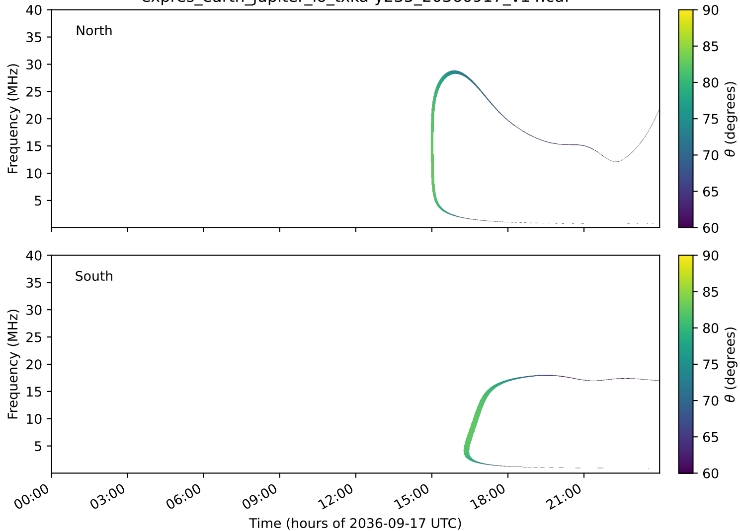
expres_earth_jupiter_io_txka-y235_20360917_v14.cdf
