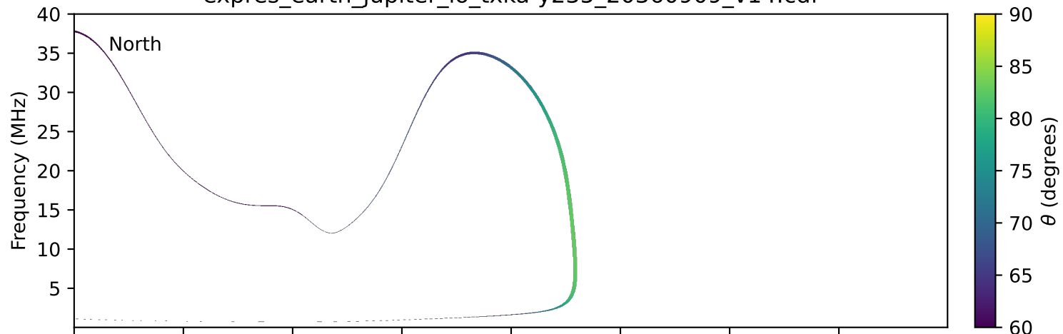
expres_earth_jupiter_io_txka-y235_20360909_v14.cdf
