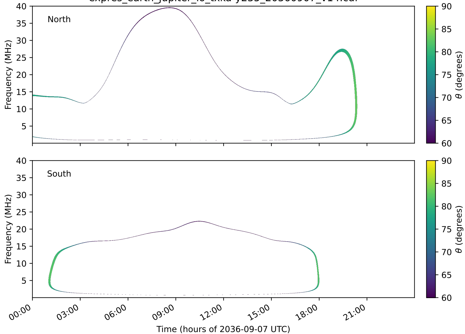
expres_earth_jupiter_io_txka-y235_20360907_v14.cdf
