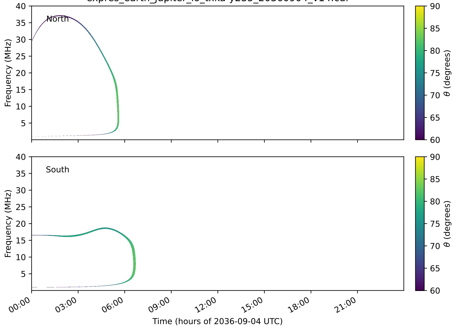
expres_earth_jupiter_io_txka-y235_20360904_v14.cdf
