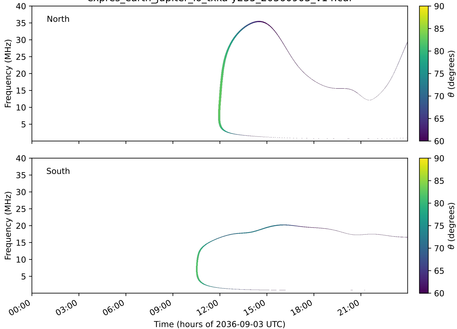
expres_earth_jupiter_io_txka-y235_20360903_v14.cdf
